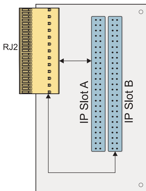
Figure 1-1 : Block Diagram
