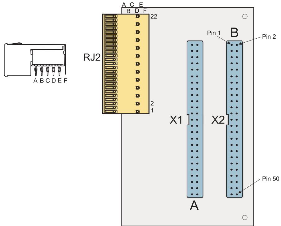
Figure 6-1 : Pin Assignment
