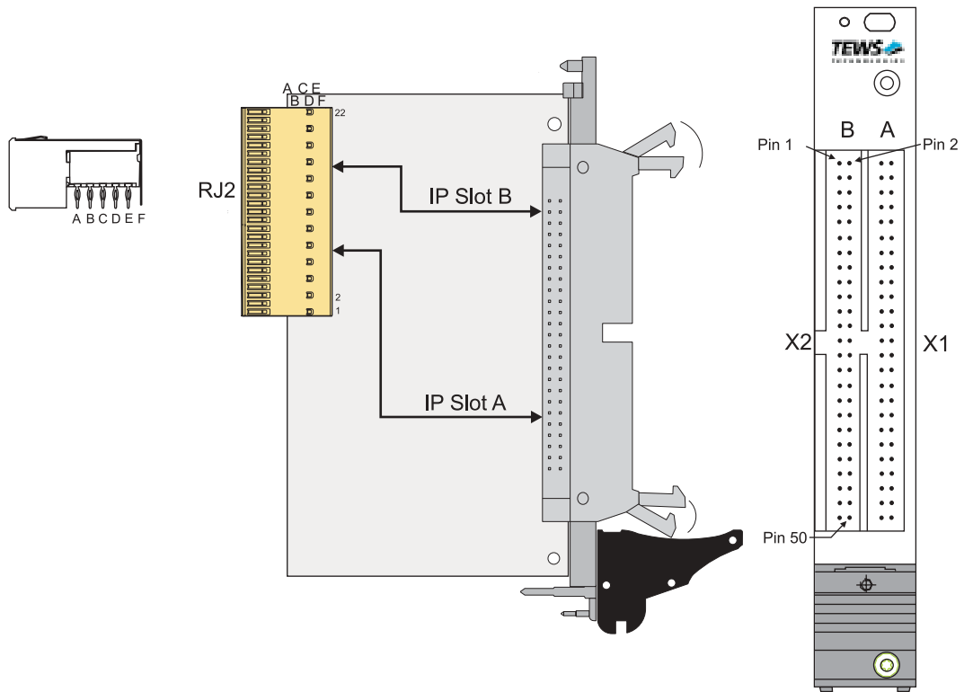
Figure 6-1 : Pin Assignment
