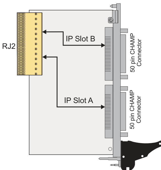
Figure 1-1 : Block Diagram
