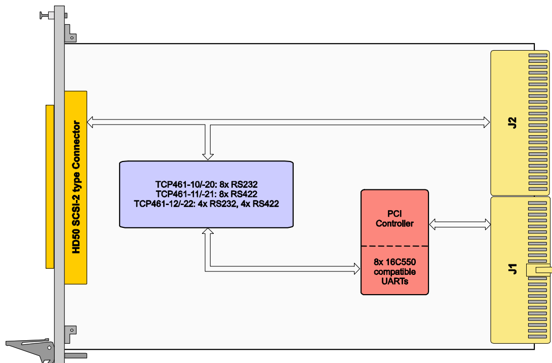
Figure 1-1 : Block Diagram
