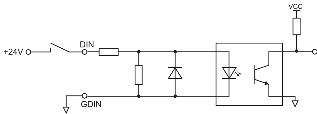
Figure 7-8 : Digital Input Wiring
